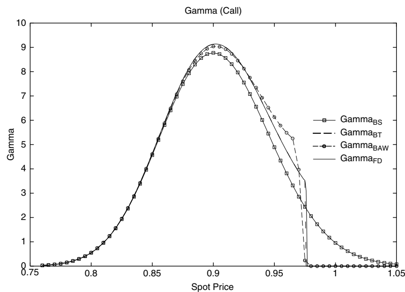
Figure 4: Gamma of an American call with K = .9 , T = 3m , r_d = .02 , r_f = .035 , \sigma = .1
