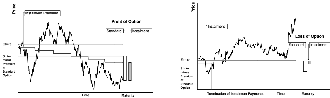
Figure 1: Comparison of two scenarios of an Instalment option. The left hand side shows a continuation of all instalment payments until expiration. The right hand side shows a scenario where the Instalment option is terminated after the first decision date.
